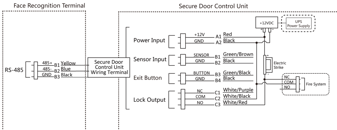
Figure 4-8 Wiring Diagram
