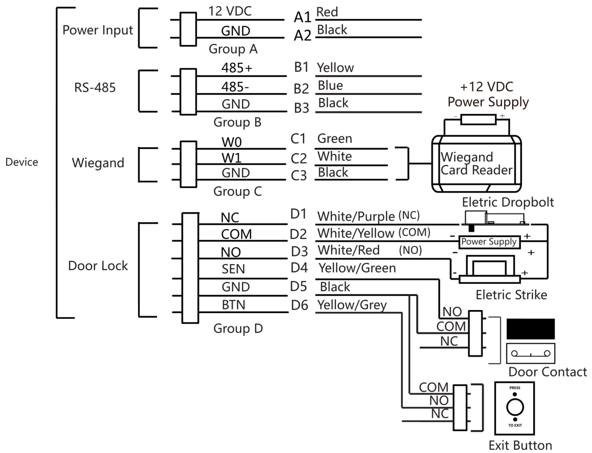
Figure 4-1 Device Wiring
