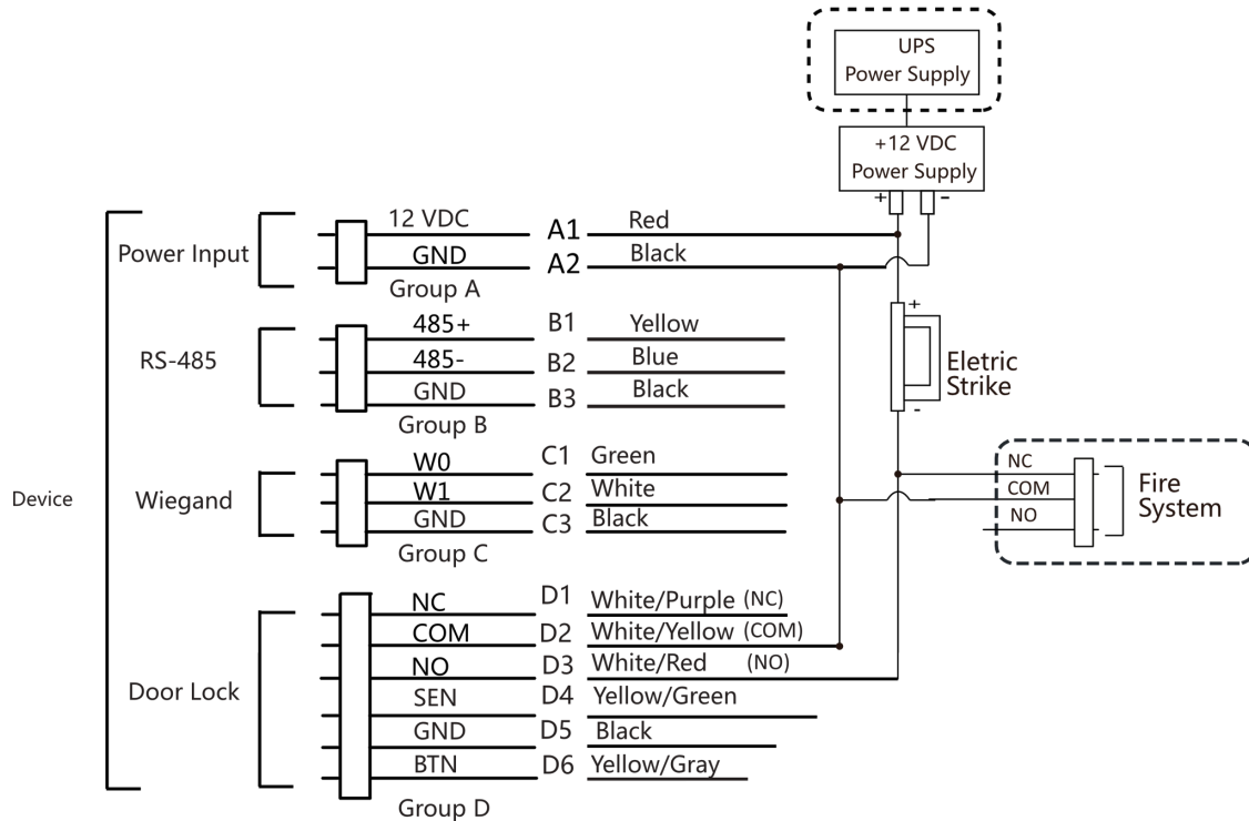
Figure 4-7 Device Wiring
