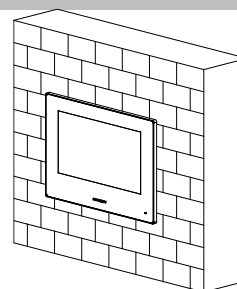
Surface Mounting
