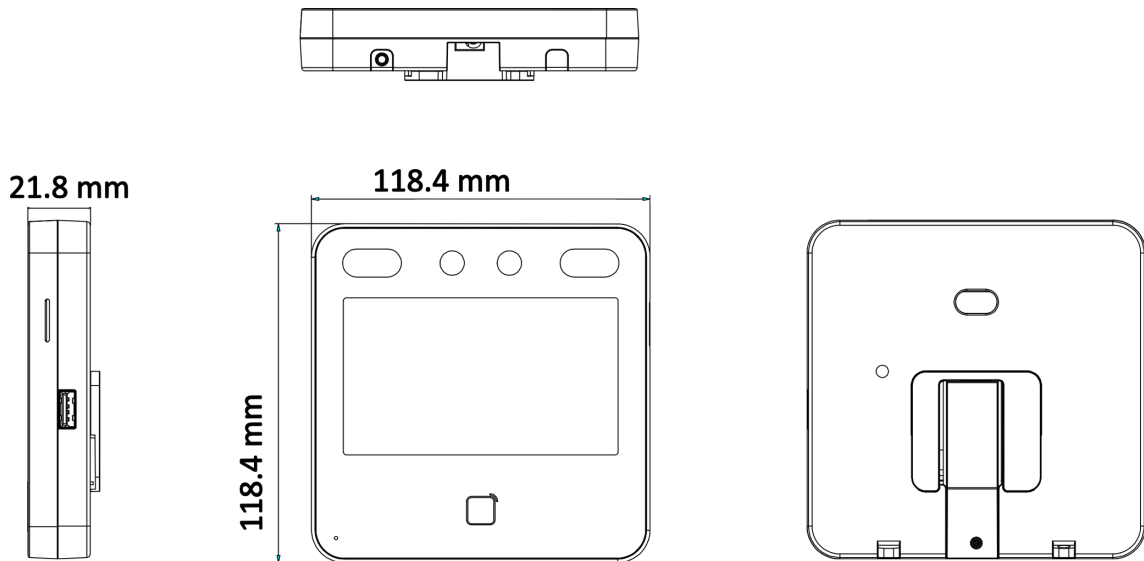
Figure D-2 Dimension (Without Fingerprint)
