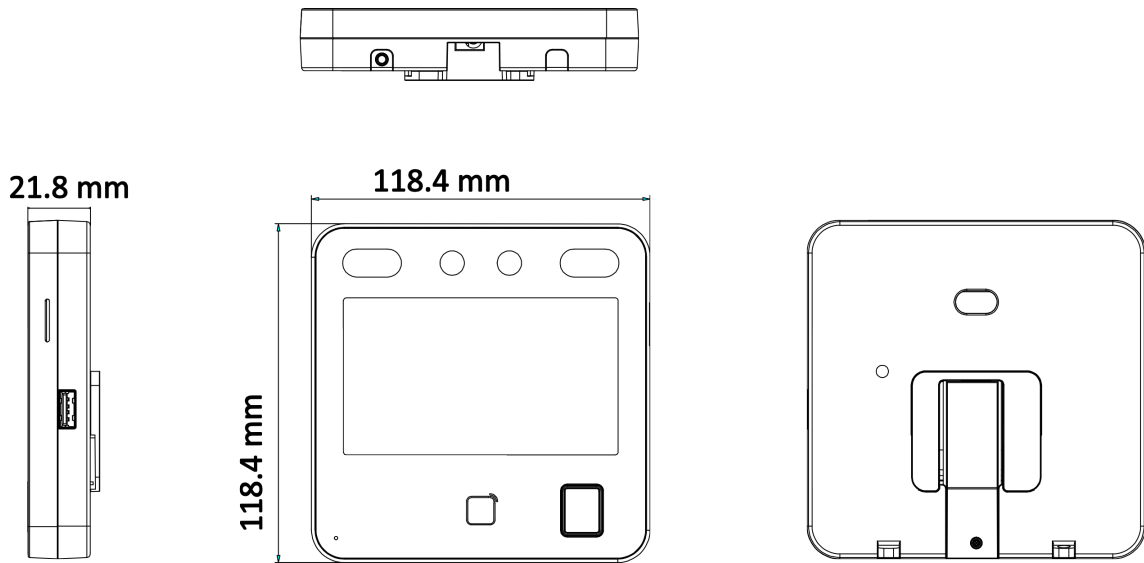
Figure D-1 Dimension (With Fingerprint)
