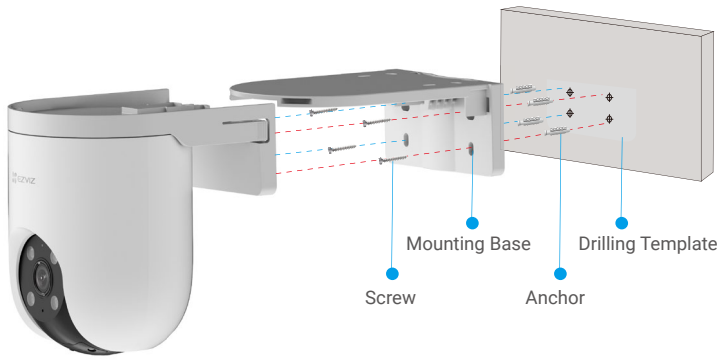
Fig. 2 Wall Mount
